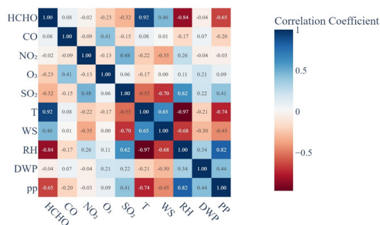
Fig. 5. Heatmap and summary of Spearman's rank coefficient for correlations between monthly average HCHO, other air pollutants ( \text{CO} , \text{NO}_2 , \text{O}_3 , \text{SO}_2 ) and Meteorological parameters (T, WS, RH, DWP, PP) in Ahvaz, Iran, from 2019 to 2022.
